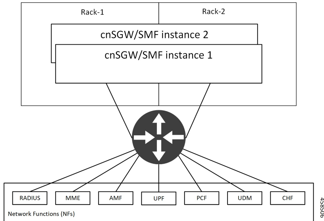
Figure 109: Active-Active Inter-Rack Redundancy Deployment
