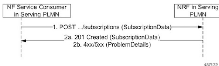
Figure 7: Subscription to NF Instances in the Same PLMN
