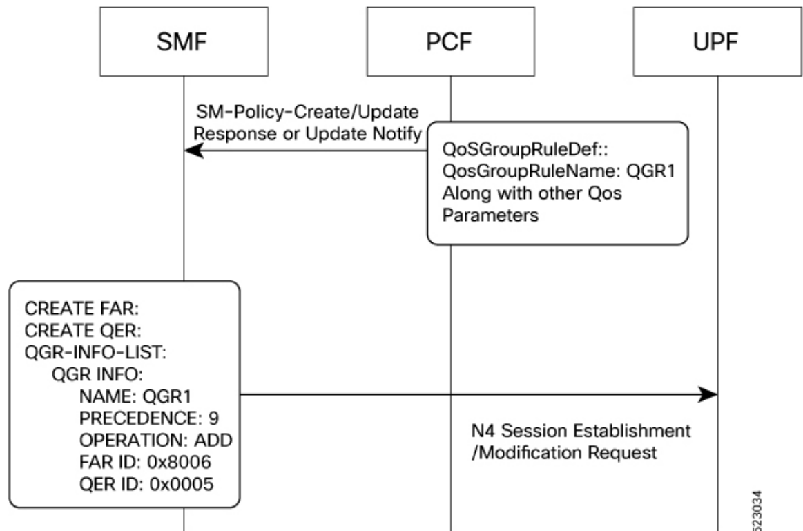
Figure 15: Qos-Group-of-Ruledef Activation Call Flow
