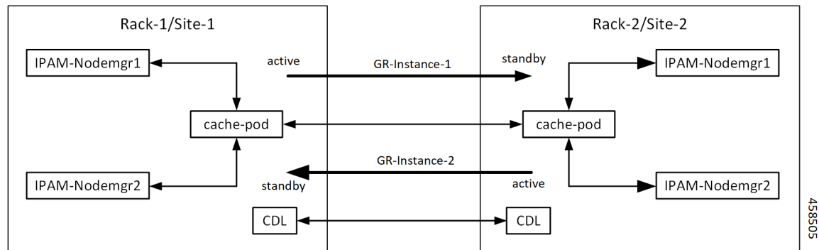
Figure 4: IPAM
