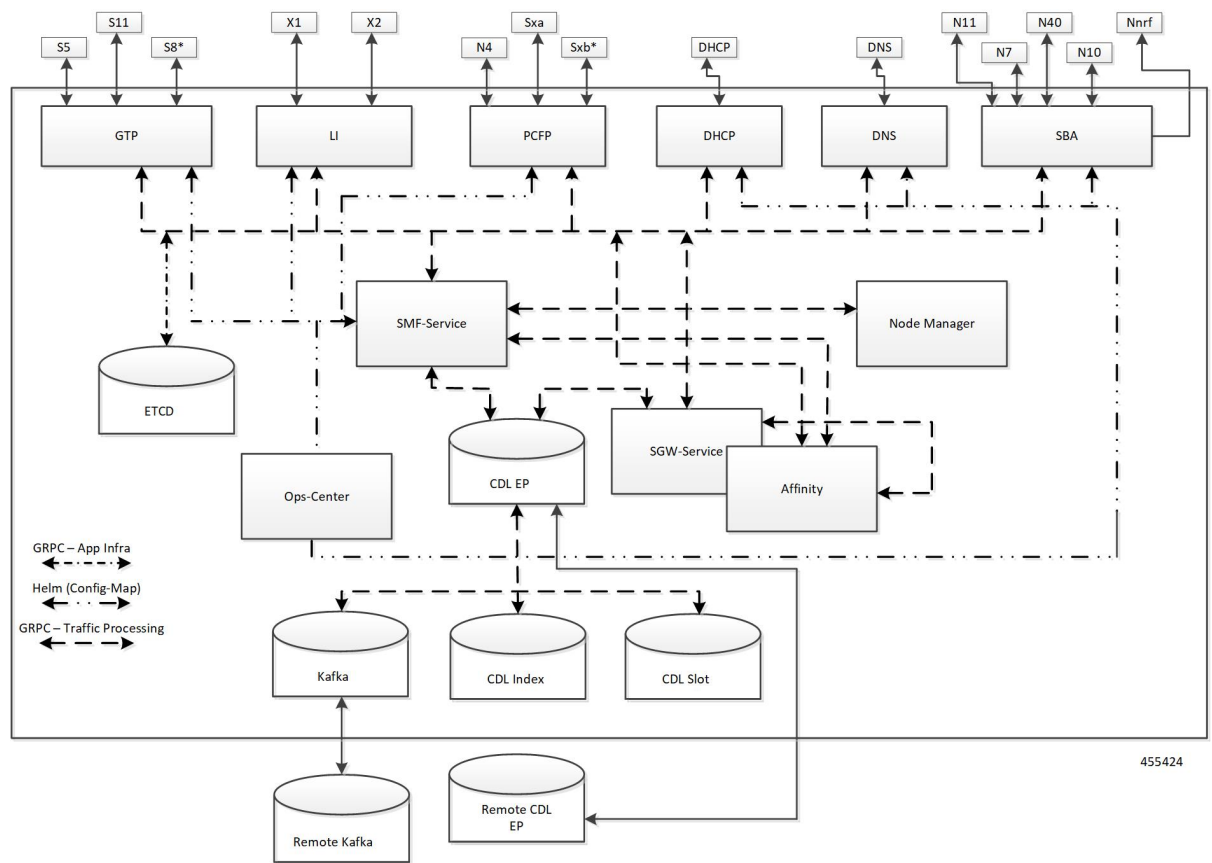
Figure 3: Kubernetes Deployment
