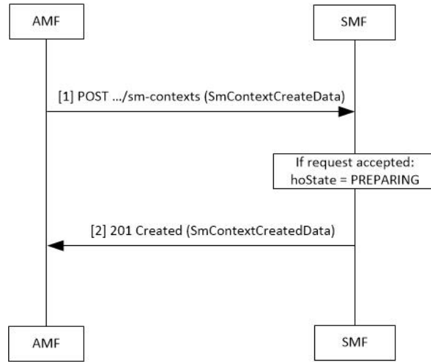
Figure 8: Flow Failure Handling Call Flow (From Source in EPS to 5GS Handover)
