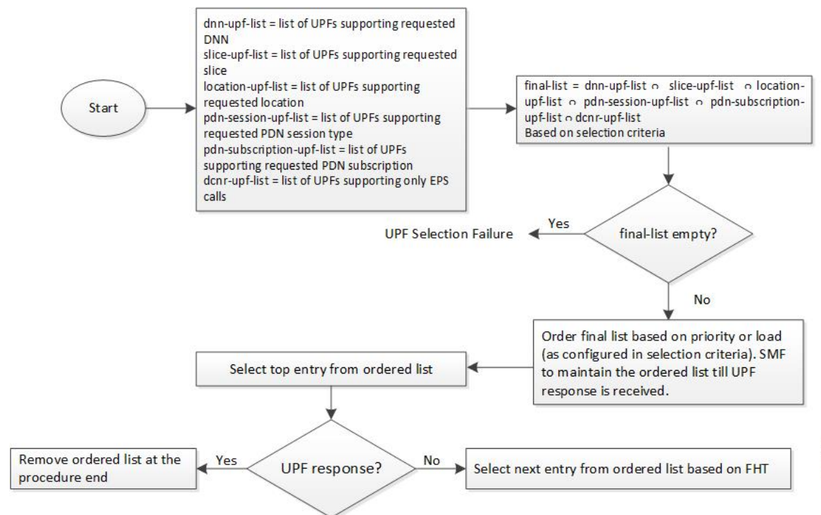
Figure 14: UPF Node Selection Workflow
