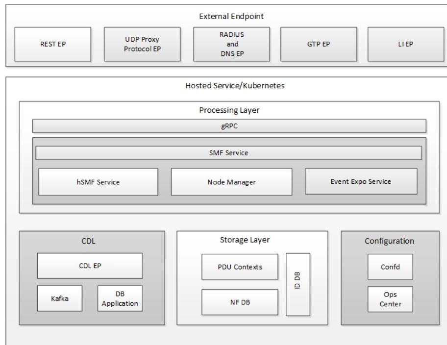
Figure 1: Communication Workflow of Pods
