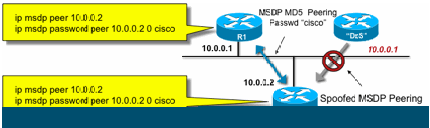
Fig. 15: MSDP MD5 Neighbor Authentication
