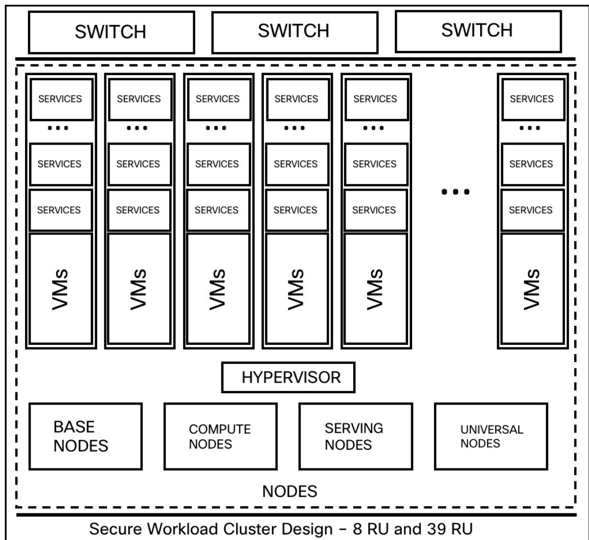
Figure 26: Conception de la conception de grappe Cisco Secure Workload
