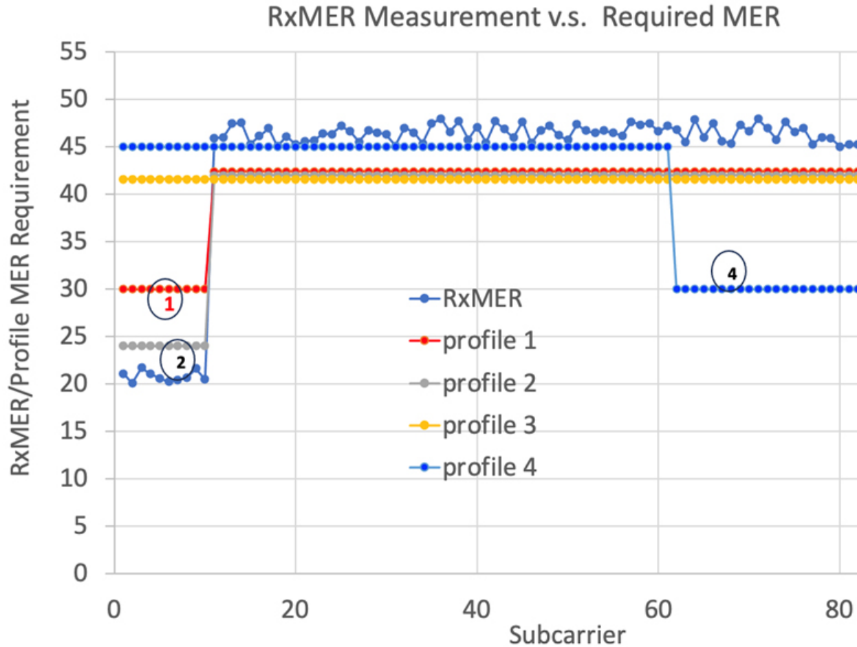
Figure 25: RxMER Measurement Against the Required MER
