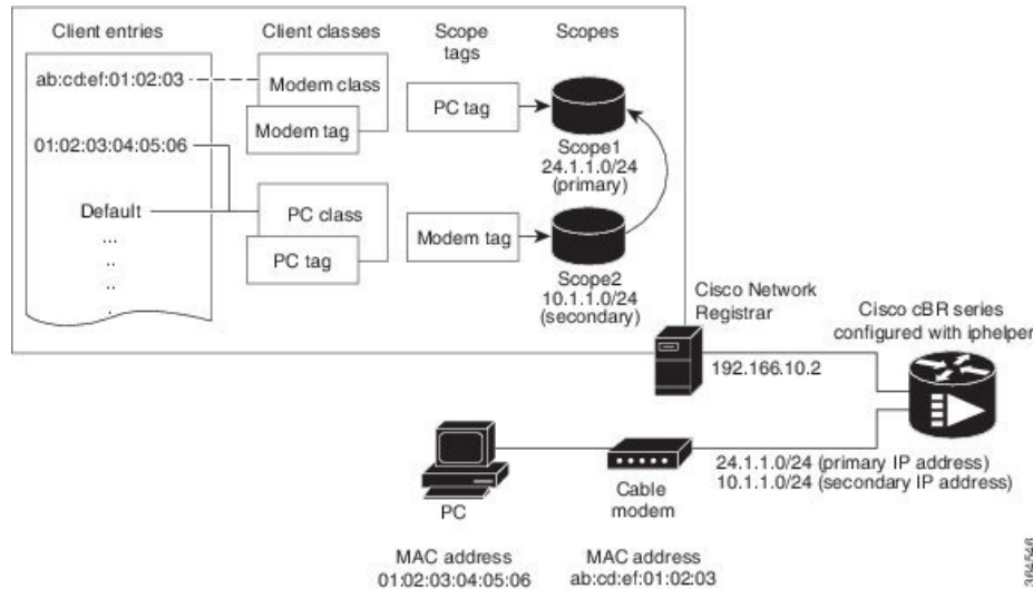
Figure 35: Trial Configuration in an HFC Network
