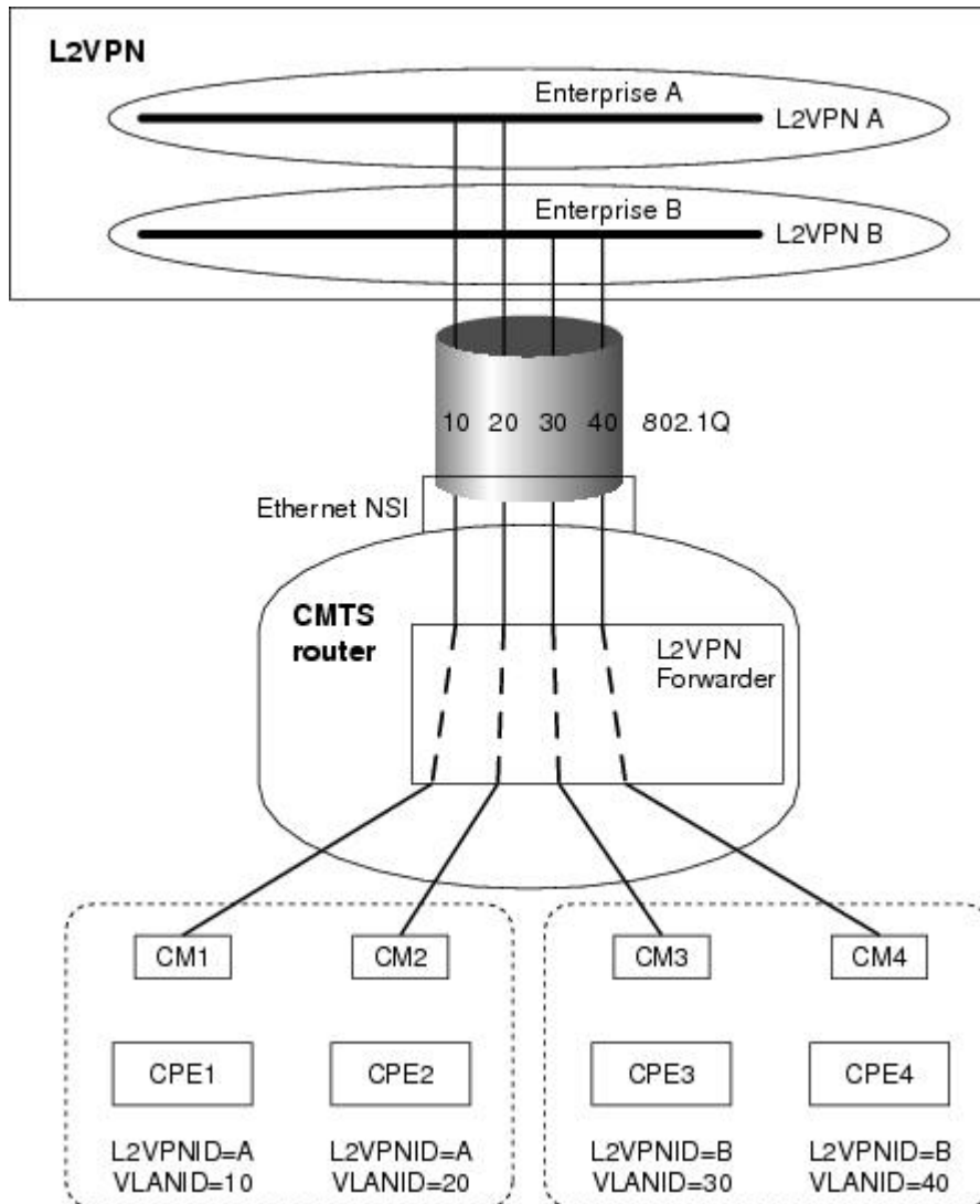
Figure 27: Point-to-Point L2VPN Network Diagram
