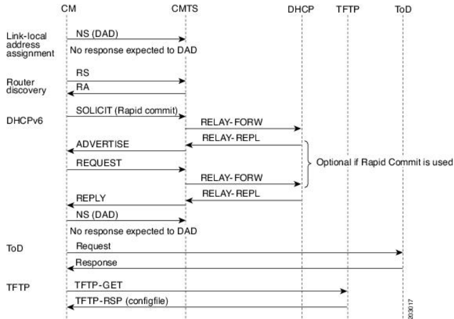
Figure 31: Message Flow for CM Provisioning of DHCP IPv6 Address Assignment
