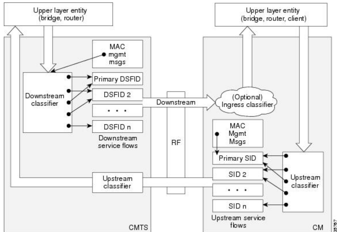
Figure 37: Classification Within the MAC Layer
