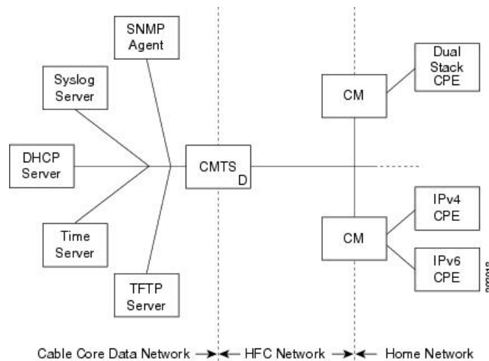
Figure 30: DOCSIS 3.0 Network Model
