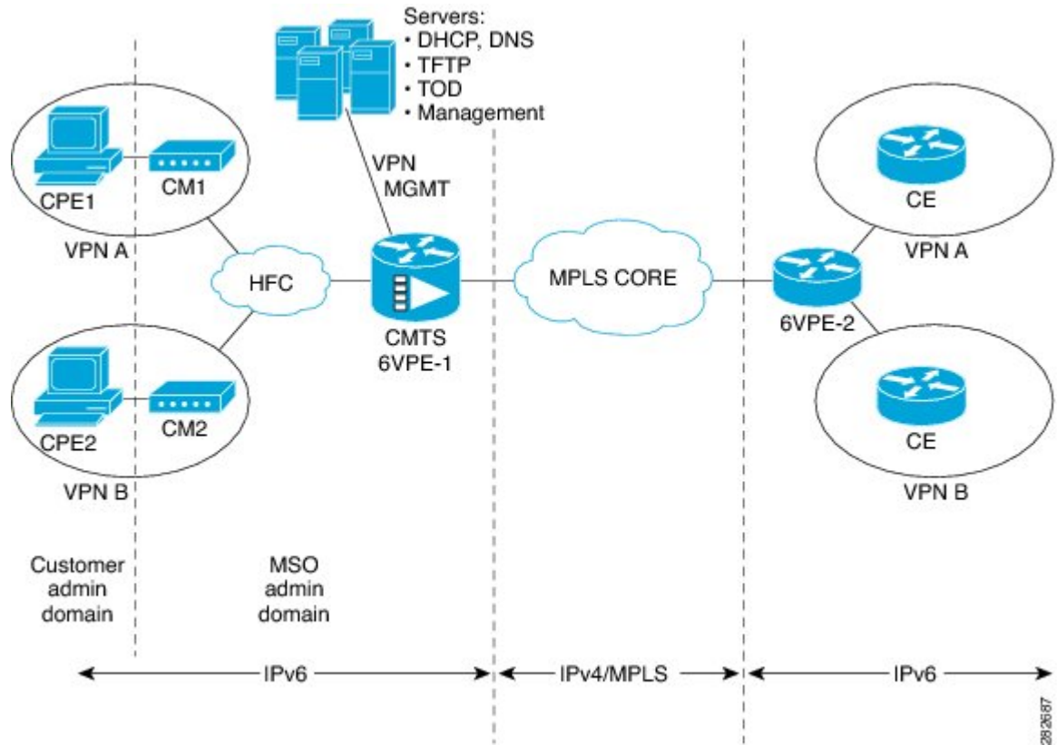
Figure 32: 6PE/6VPE Reference Architecture
