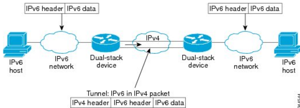
Figure 21: Overlay Tunnels
