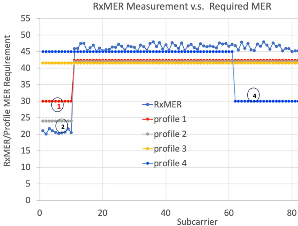
Figure 24: RxMER Measurement Against the Required MER
