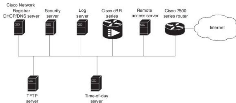
Figure 34: Servers Required on a Two-Way HFC Network
