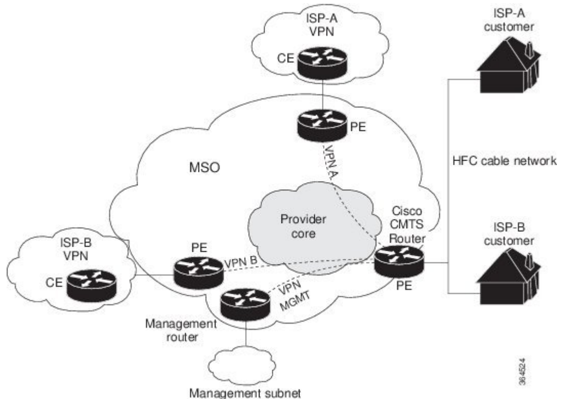
Figure 29: MPLS VPN Network
