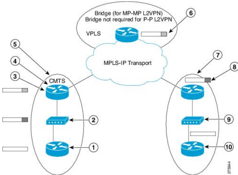
Figure 28: Transporting Layer 2 Packets
