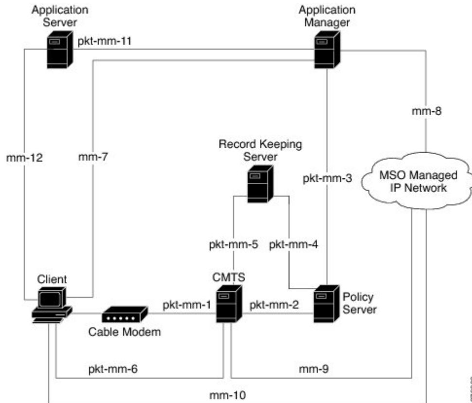
Figure 36: PCMM Architectural Overview
