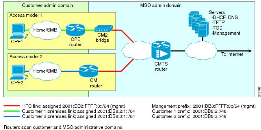
Figure 33: IPv6 CPE Router Reference Architecture
