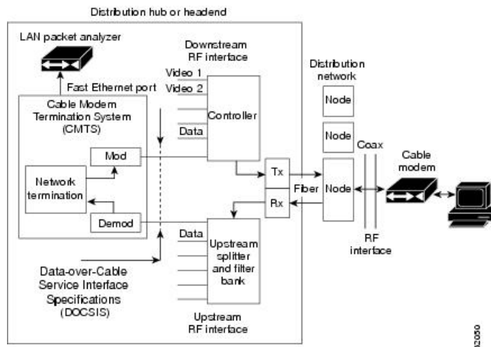
Figure 39: LAN Packet Analyzer in a DOCSIS Two-Way Configuration
