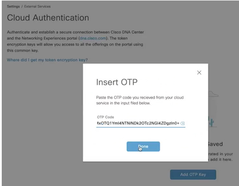
Figure 30: Register Cisco DNA Center to Cisco DNA Cloud
