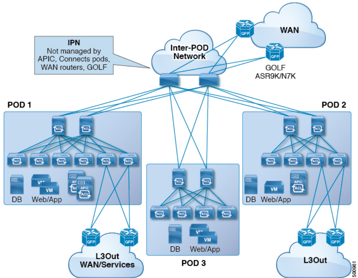
Figure 10: Multi-Pod Overview
