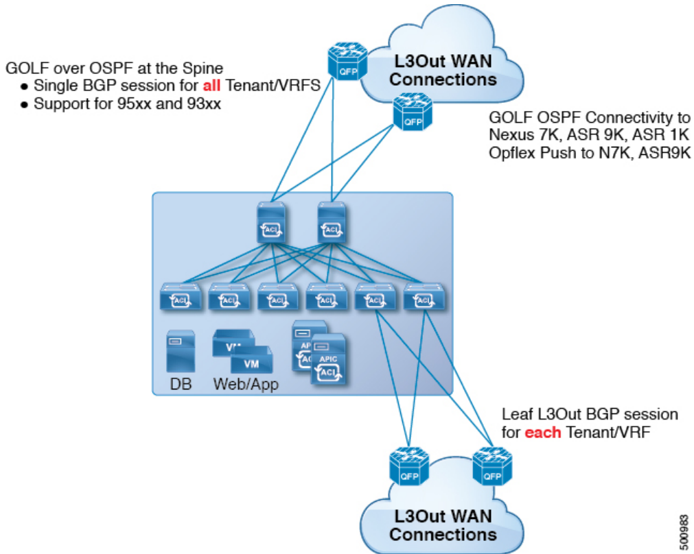
Figure 58: Cisco ACI GOLF Topology
