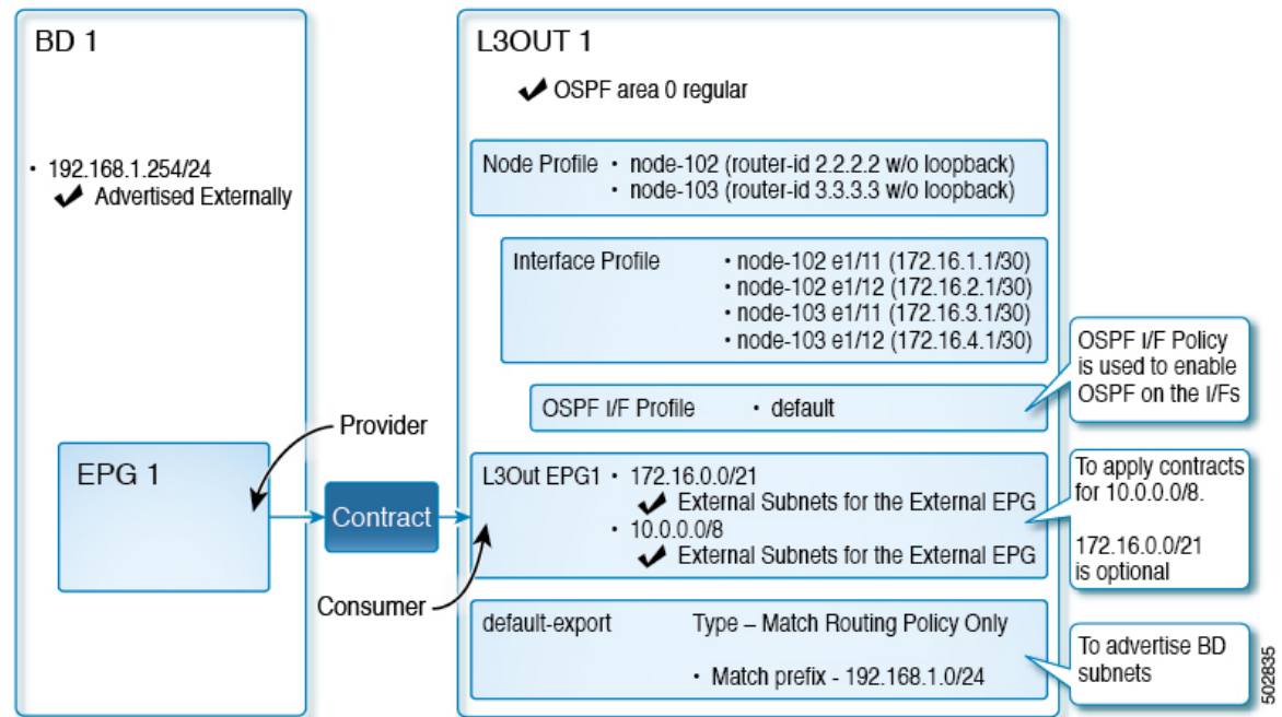
Figure 31: OSPF Configuration Diagram
