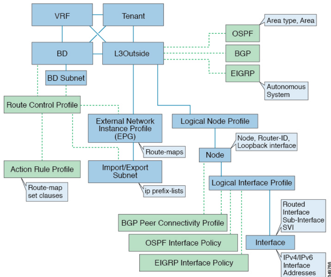
Figure 27: ACI Layer 3 Managed Objects
