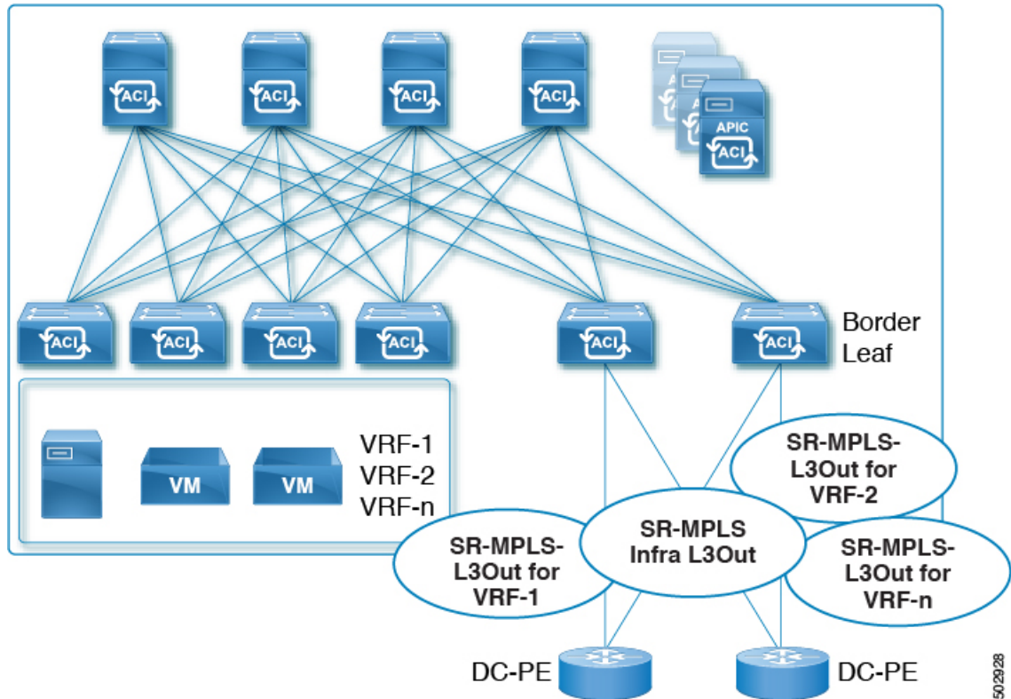
Figure 20: User Tenant SR-MPLS L3Out
