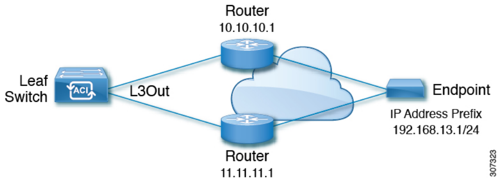
Figure 56: Example Static Route
