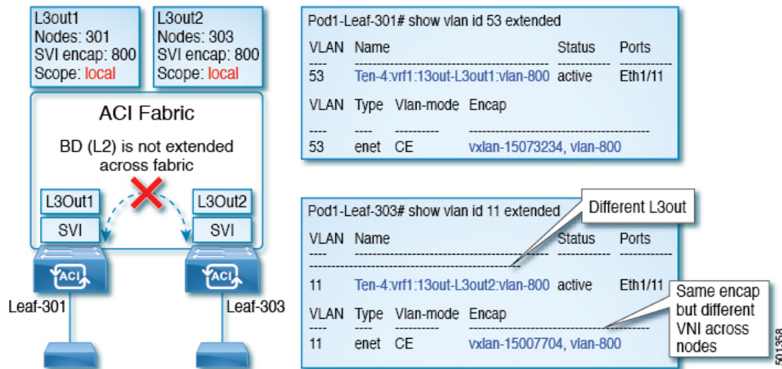
Figure 34: Local Scope Encapsulation and Two Layer 3 Outs
