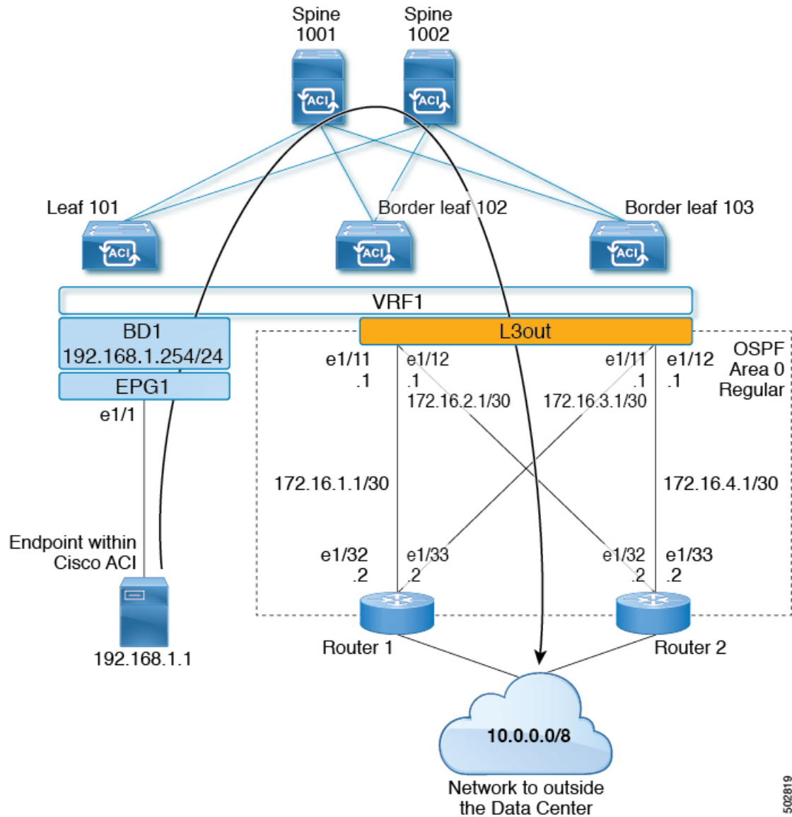
Figure 30: Example Topology for an OSPF L3Out with Two External Routers
