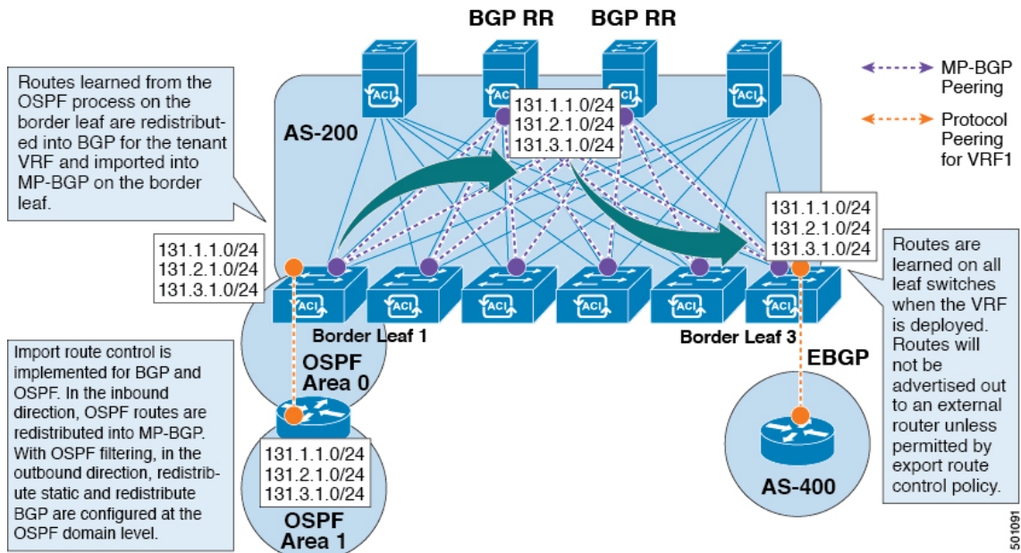
Figure 26: ACI Route Redistribution
