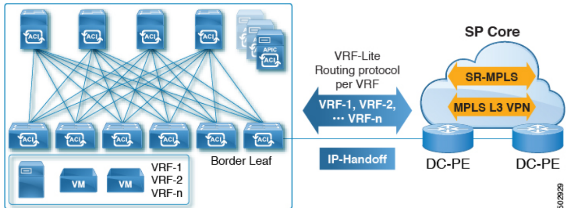
Figure 18: ACI Handoff to DC-PE Using IP Handoff (VRF-Lite)
