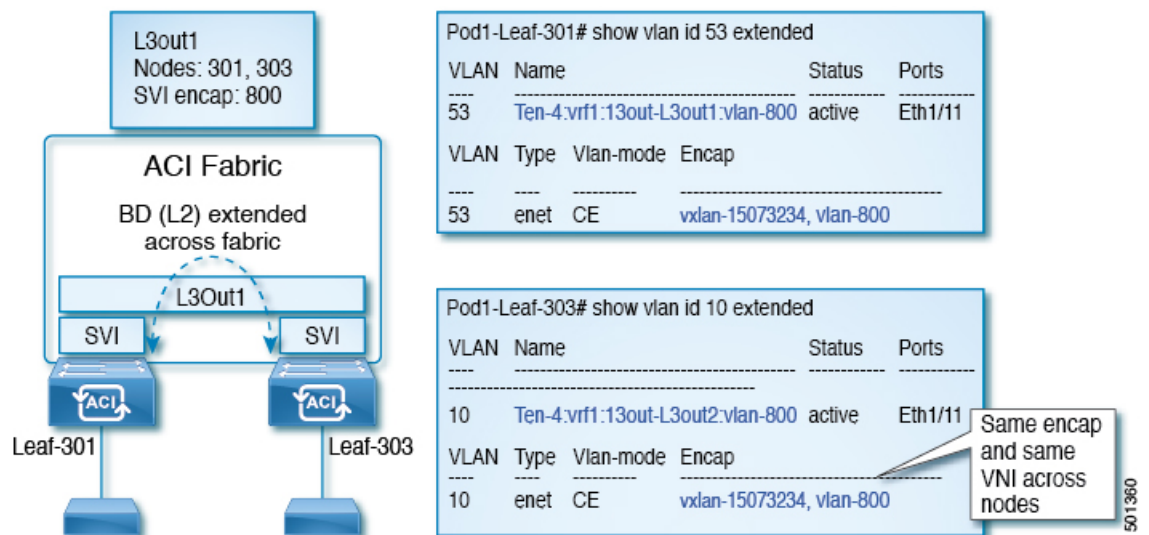
Figure 33: Local Scope Encapsulation and One Layer 3 Out
