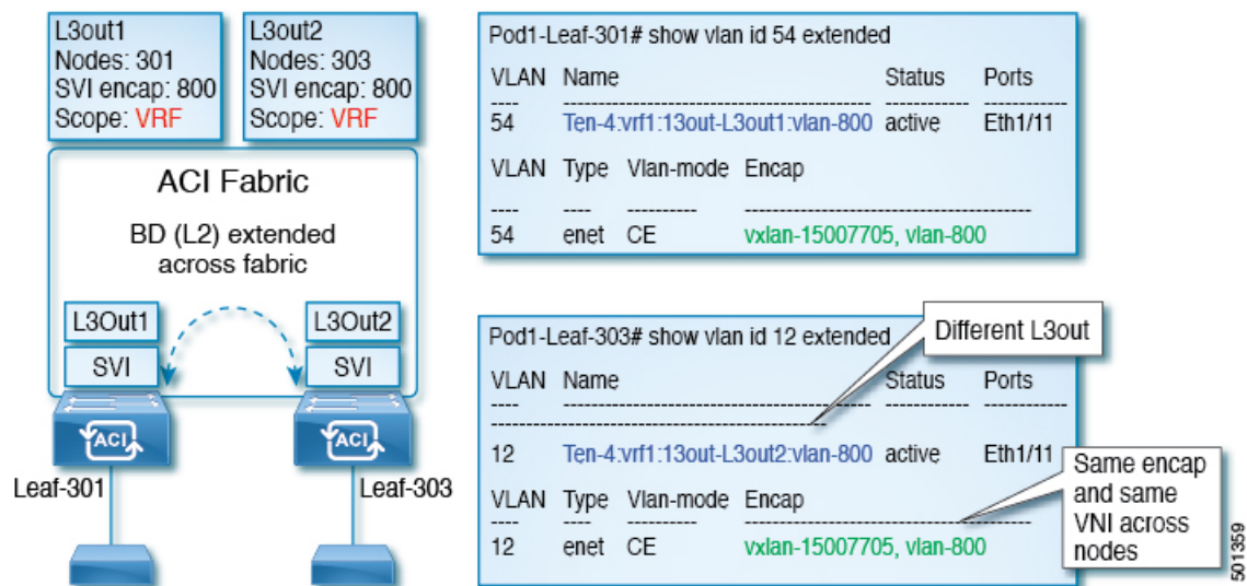
Figure 35: VRF Scope Encapsulation and Two Layer 3 Outs
