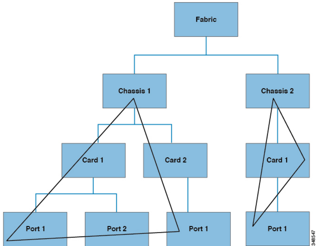
Figure 6: Tree-Level Queries
