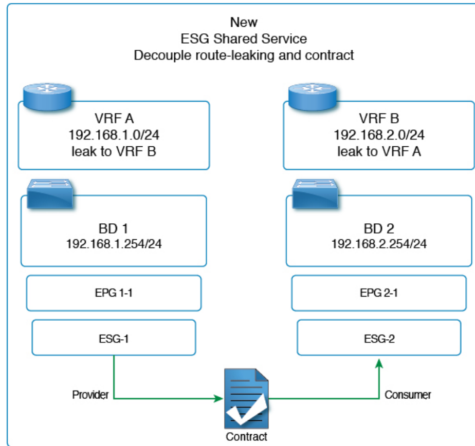
Figure 6: Route Leaking with ESGs
