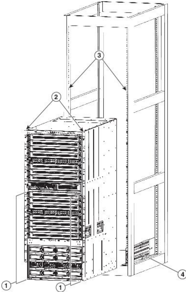
Figure 9: Moving a Chassis onto a Rack or Cabinet - Cisco MDS 9718 Chassis
