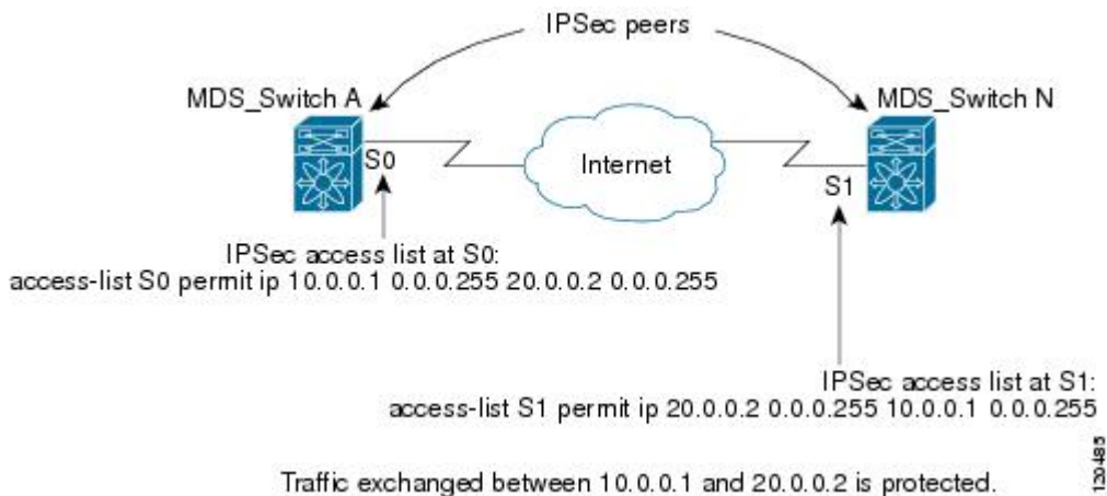
Figure 14: IPsec Processing of Crypto IPv4-ACLs
