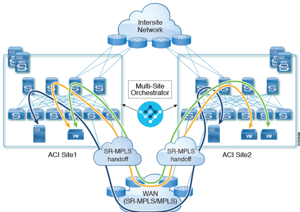
Figure 29: Multi-Site and MPLS
