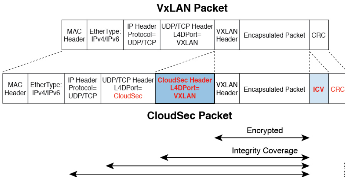
Figure 20: CloudSec Packet
