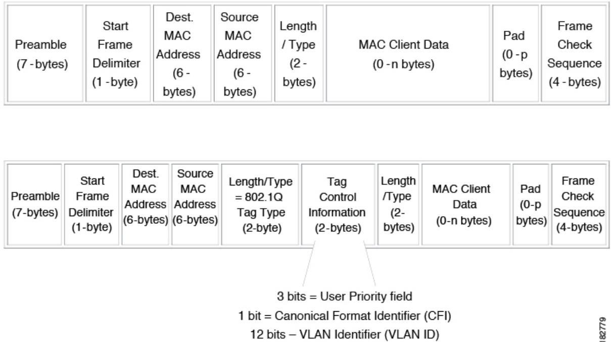
Figure 5: Header Without and With 802.1Q Tag Included
