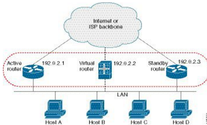
Figure 21: HSRP Topology with Two Enabled Routers
