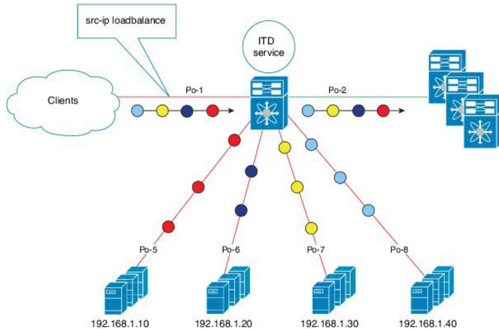
Figure 13: One-Arm Deployment Mode
