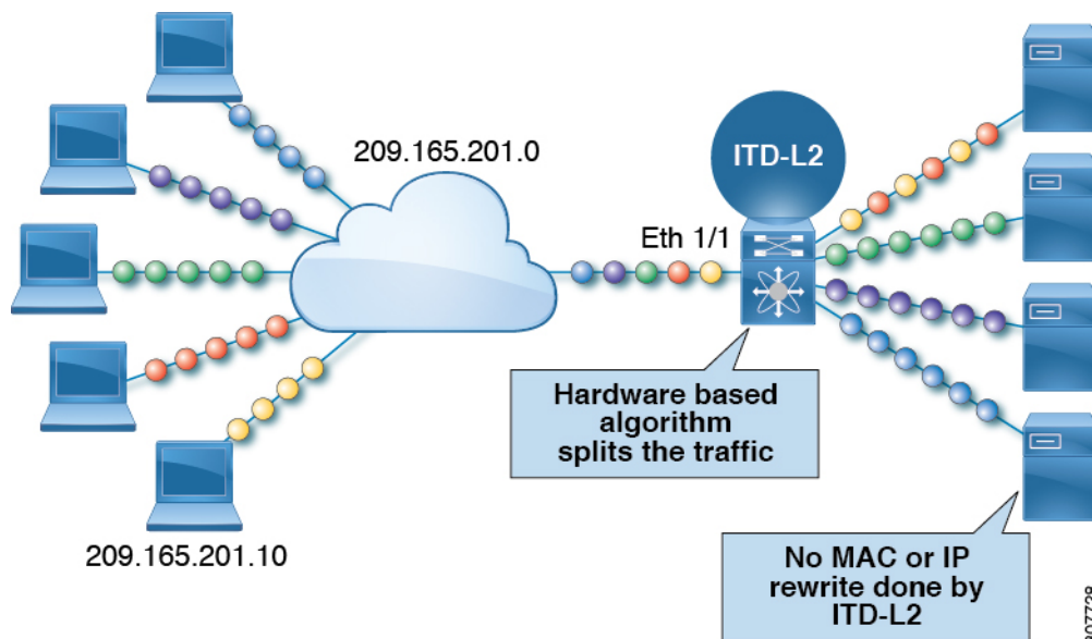
Figure 8: Standard Topology for Layer-2 load balancing
