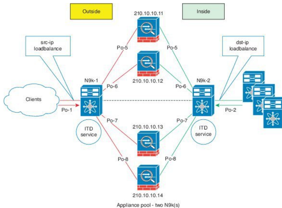
Figure 15: Sandwich Deployment Mode
