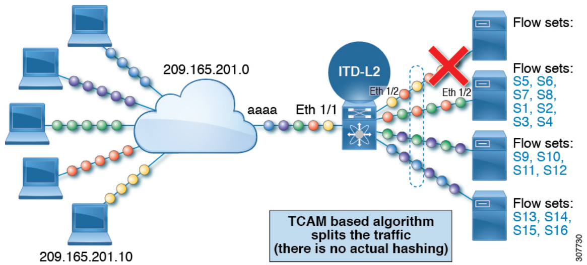
Figure 10: Fail-Action of a ITD-L2 Configuration
