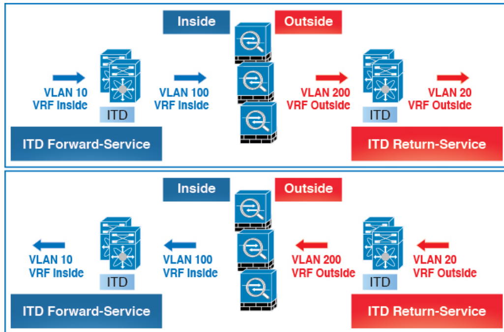
Figure 19: ITD ASA Deployment
