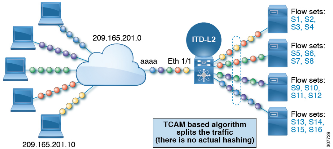
Figure 9: Use Case for a Layer-2 load balancing Configuration
