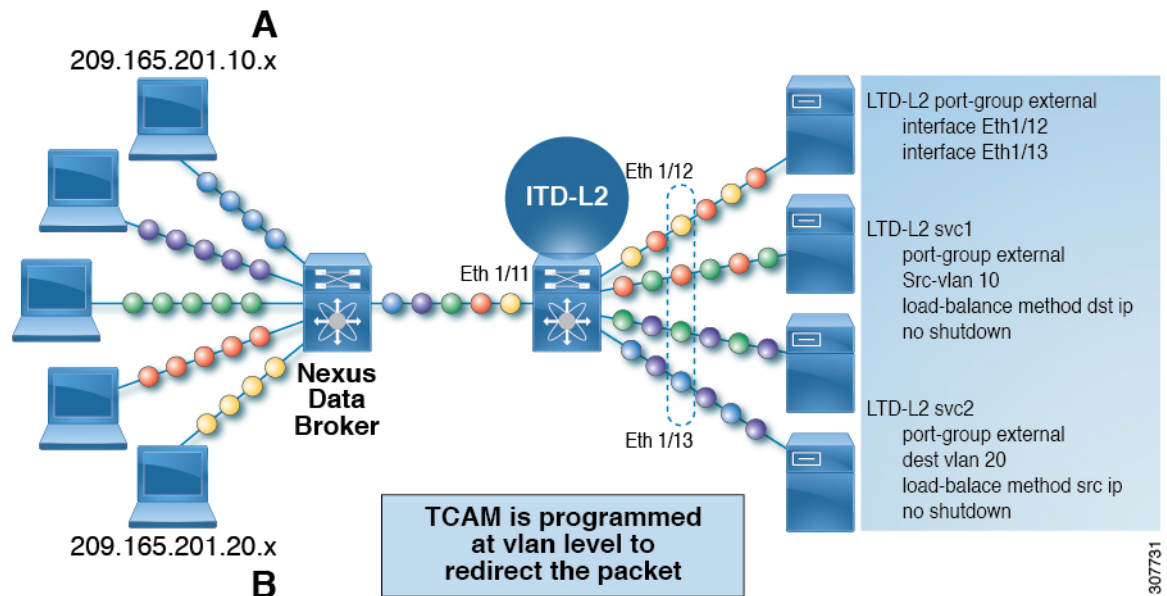
Figure 11: Fail-Action of a ITD-L2 Configuration with Resilient Hashing
