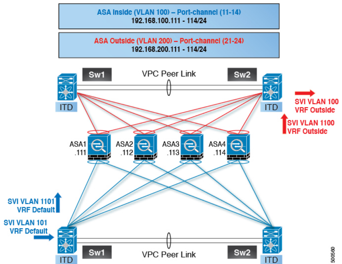
Figure 23: Dual-Switch Sandwich Mode with vPCs
