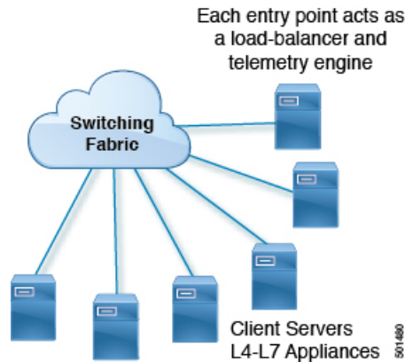
Figure 6: Load Balancing across the Fabric
