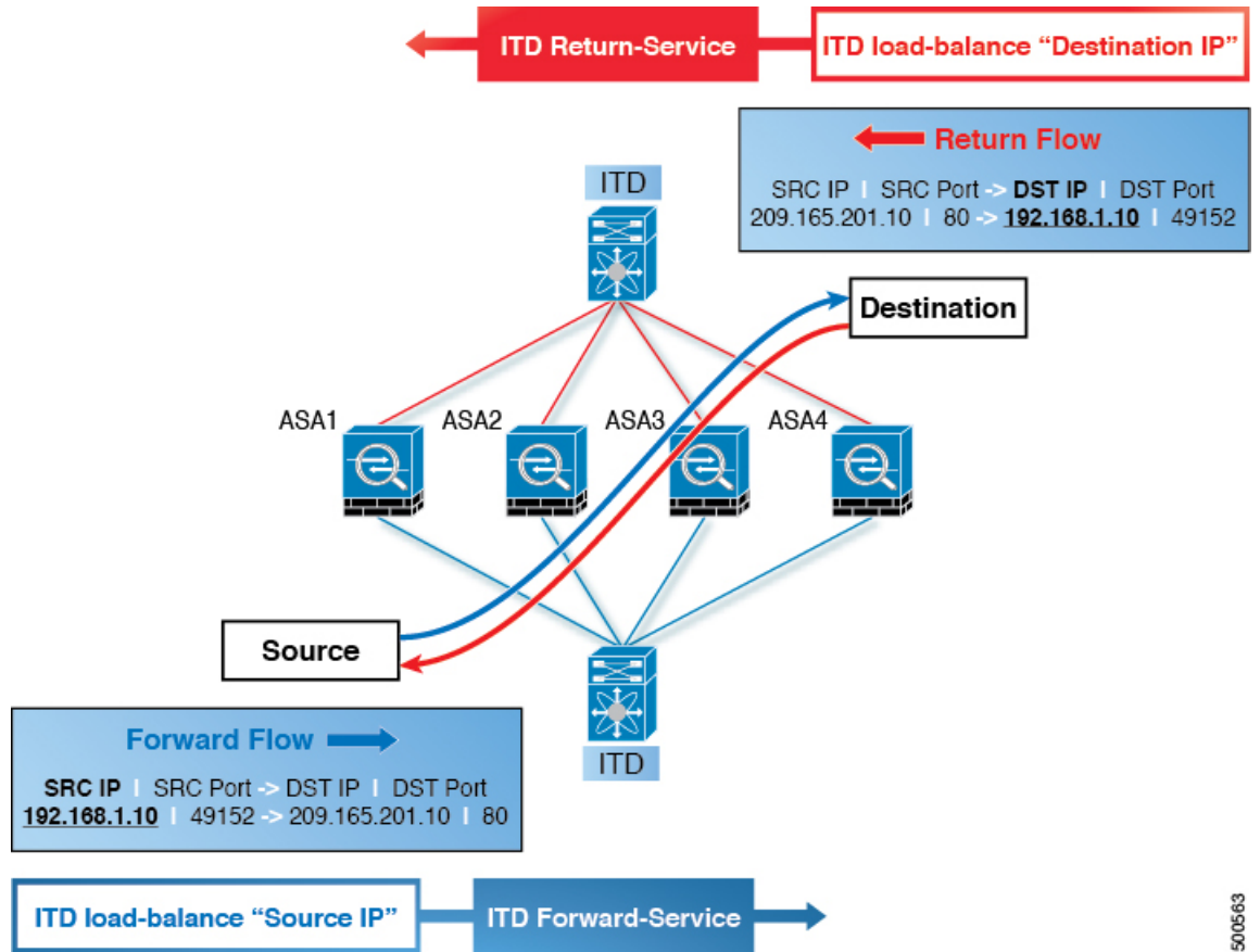
Figure 20: Flow Symmetry in ITD ASA Deployment
