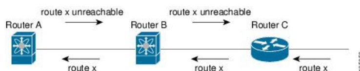
Figure 33: RIP with Split Horizon Poison Reverse
