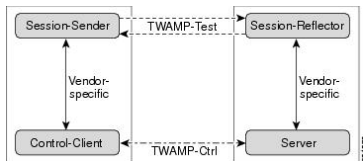
Figure 11: TWAMP Architecture
