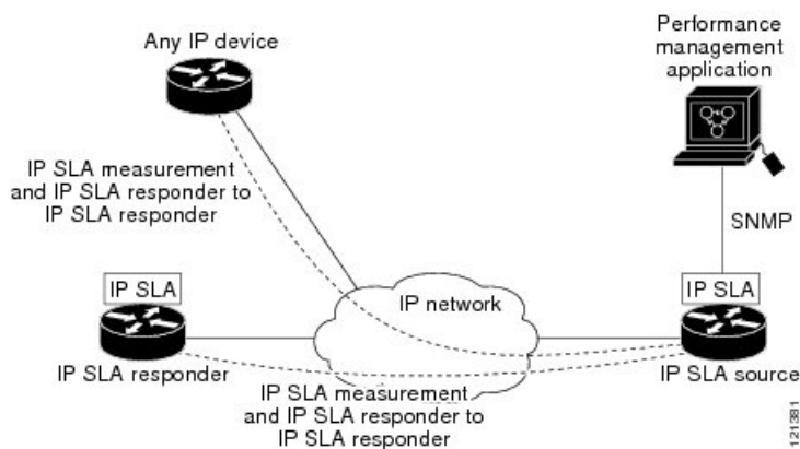
Figure 2: Cisco NX-OS IP SLAs Operations
