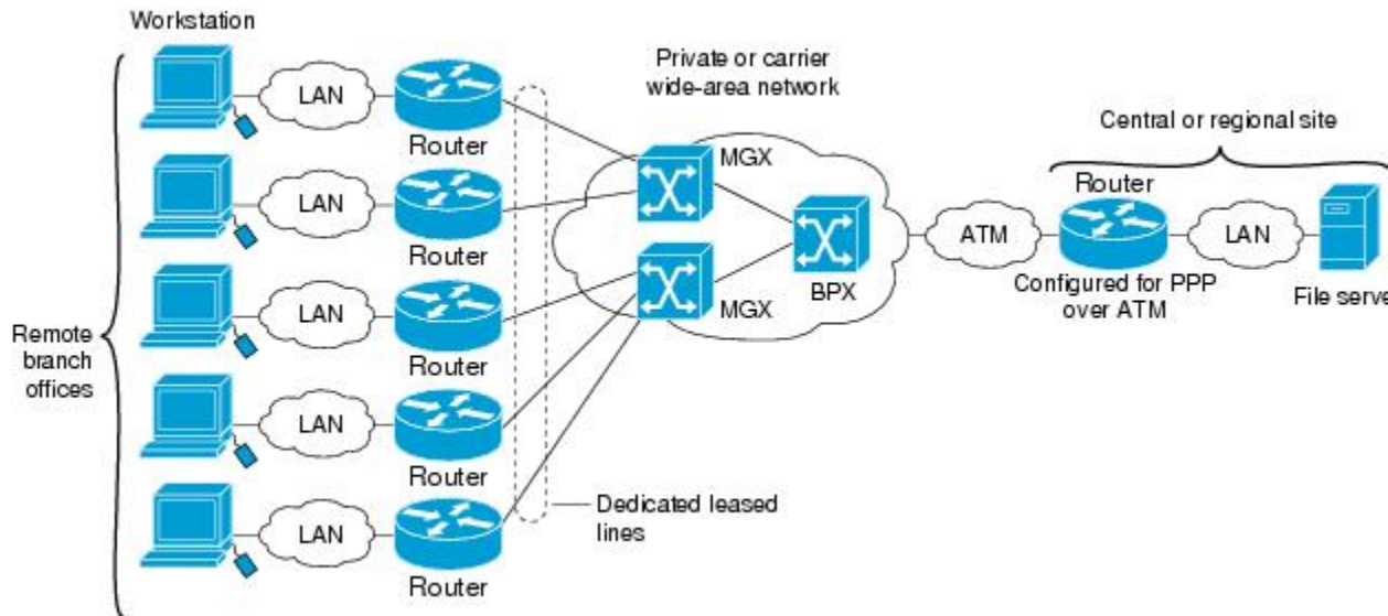
Figure 1 PPP-over-ATM Network Environment
