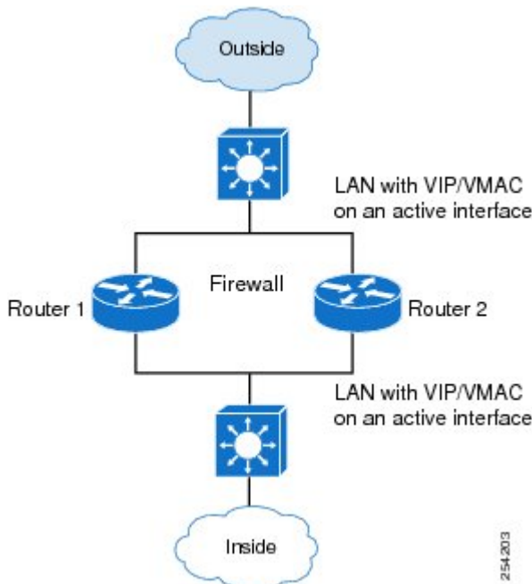
Figure 16: LAN-LAN Scenario
