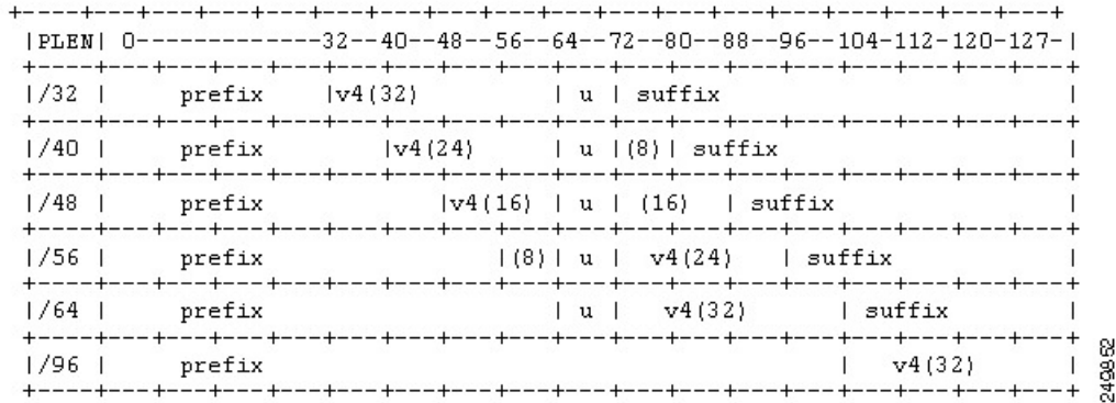
Figure 12: IPv4-Translatable IPv6 Address Format
