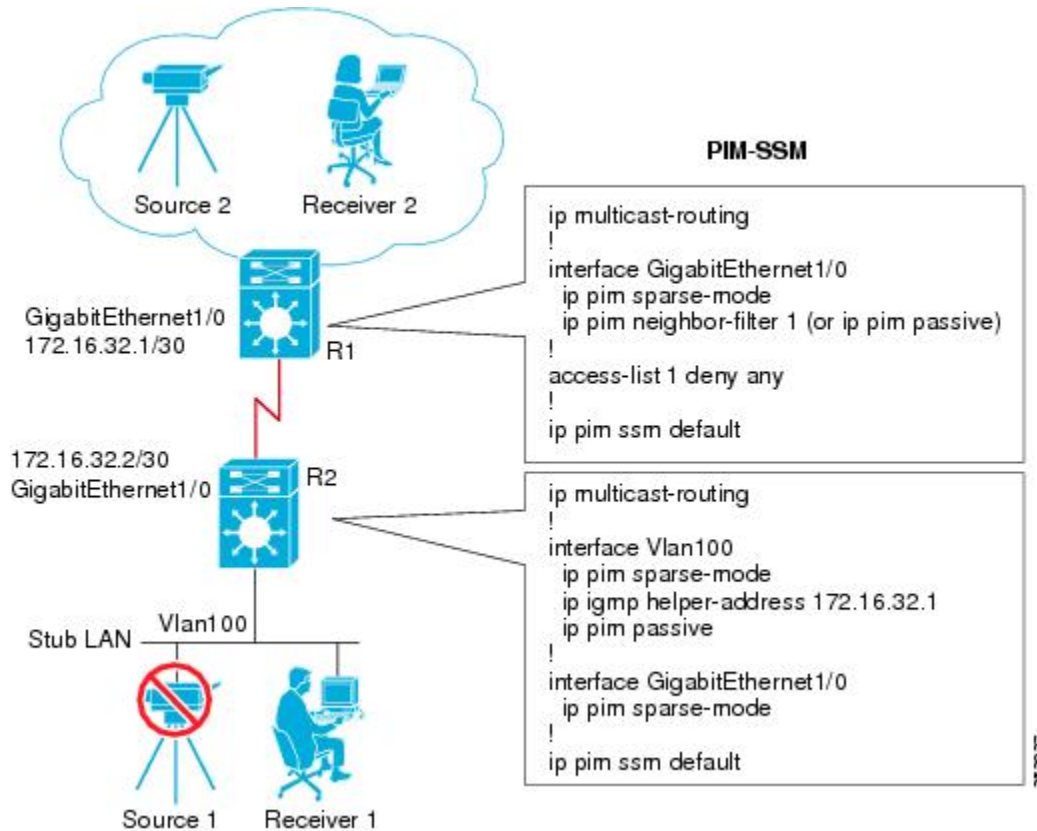
Figure 14 Multicast Stub Routing Example Topology (PIM-SSM)
