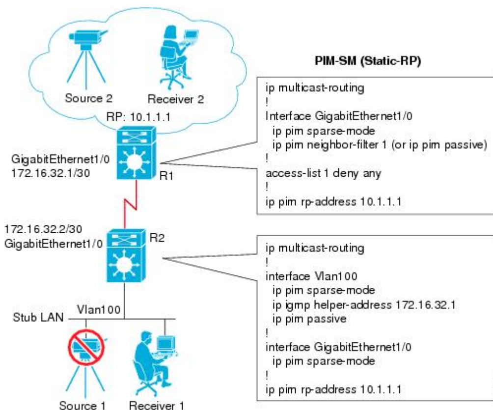
Figure 13 Multicast Stub Routing Example Topology (PIM-SM, Static RP)
