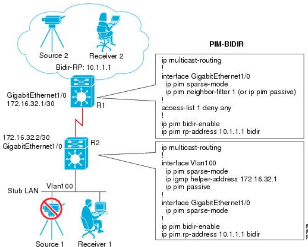
Figure 15 Multicast Stub Routing Example Topology (Bidir-PIM)
