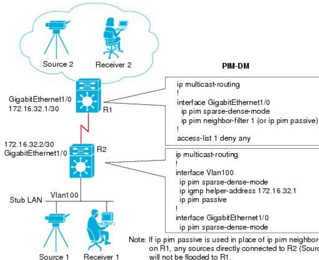
Figure 12 Multicast Stub Routing Example Topology (PIM-DM)
