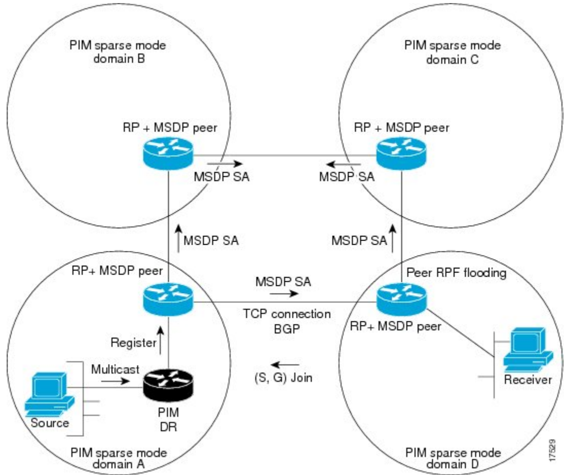
Figure 10: MSDP Running Between RP Peers
