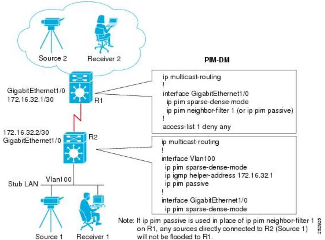
Figure 13: Multicast Stub Routing Example Topology (PIM-DM)
