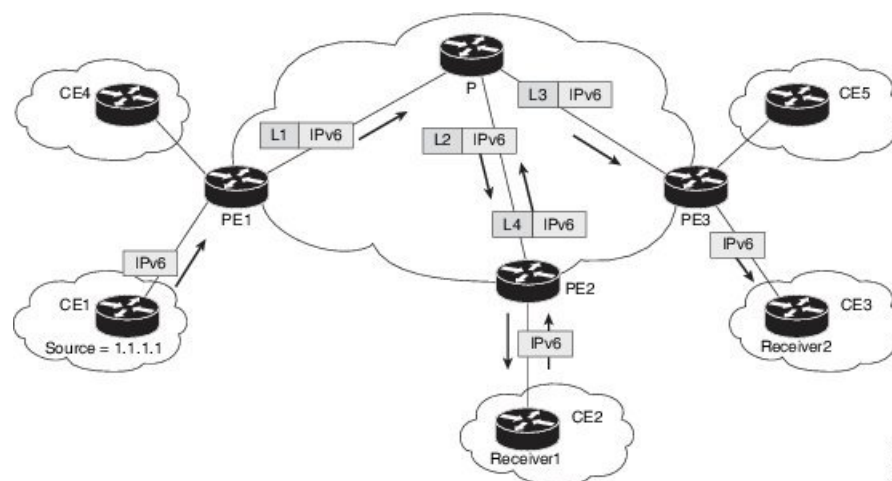
Figure 10: mLDpv6 topology
