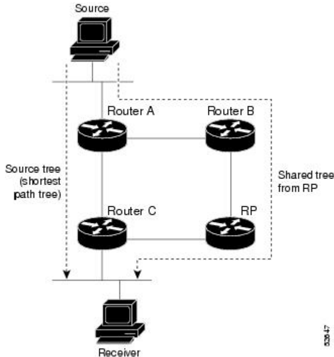
Figure 19: Shared Tree and Source Tree (Shortest Path Tree)
