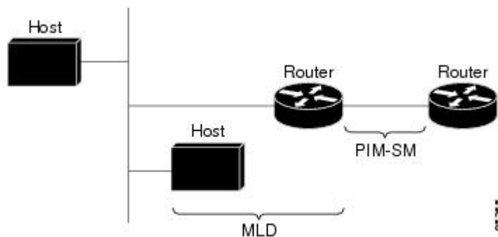
Figure 18: IPv6 Multicast Routing Protocols Supported for IPv6
