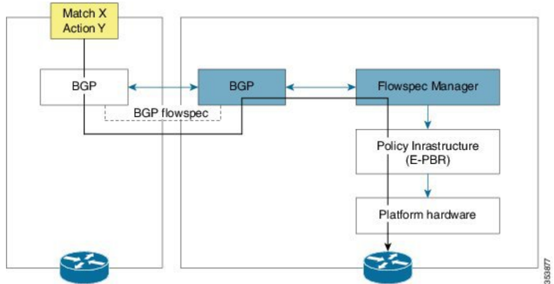
Figure 1: BGP Flow Specification Model
