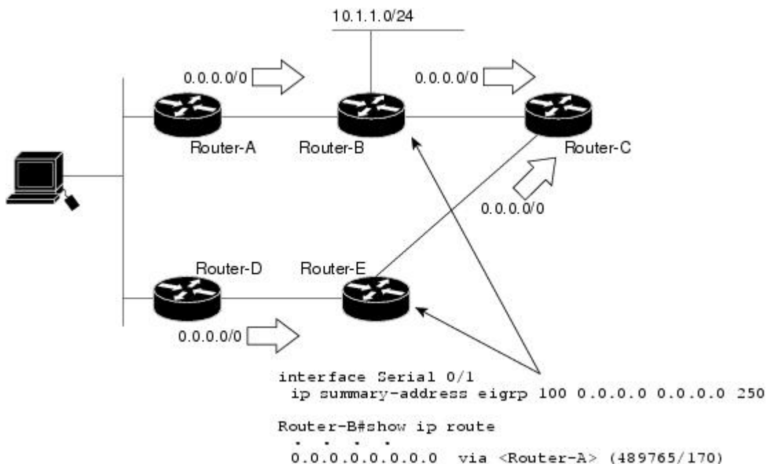
Figure 2: Floating Summary Route Applied for Dual-Homed Remotes
