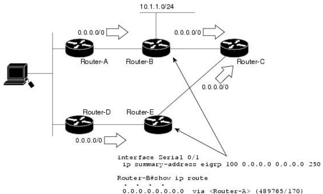
Figure 9: Floating Summary Route Applied for Dual-Homed Remotes
