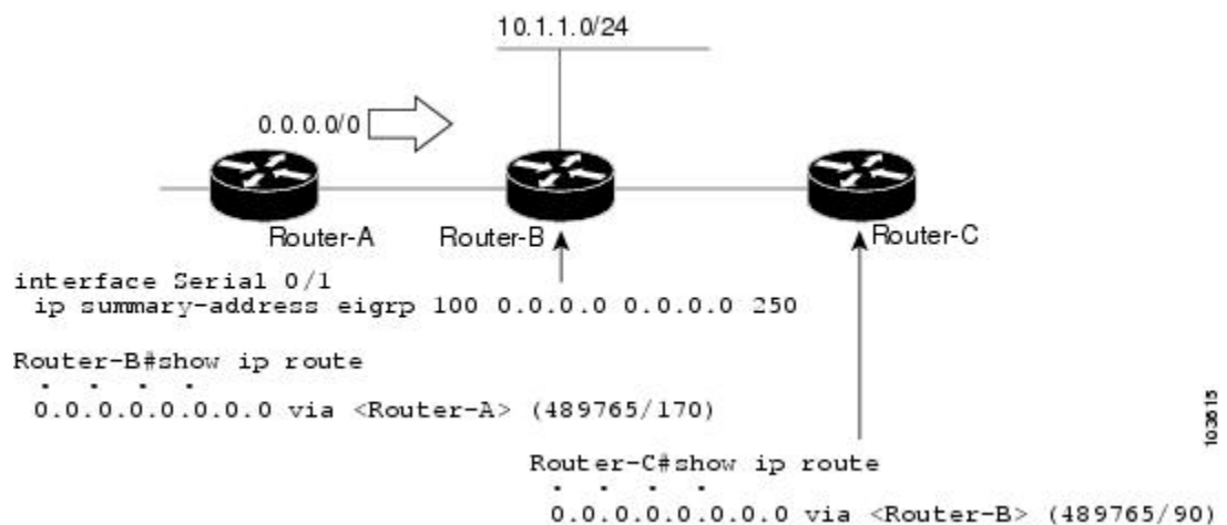
Figure 8: Floating Summary Route Applied to Device-B
