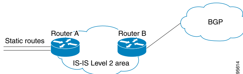
Figure 6 Example of Redistributing IS-IS Routes Using a Route Map
