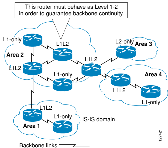
Figure 2 Level 1, Level 2, and Level 1-2 Routers in an IS-IS Network Topology
