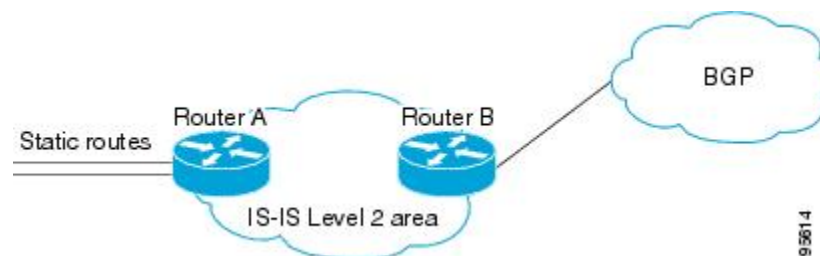
Figure 6 Example of Redistributing IS-IS Routes Using a Route Map
