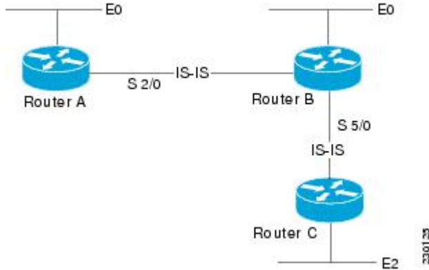
Figure 5 IS-IS Routing
