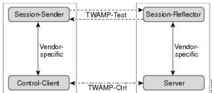
Figure 24: TWAMP Architecture
