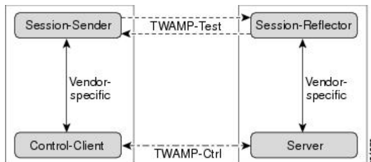
Figure 1: TWAMP Architecture
