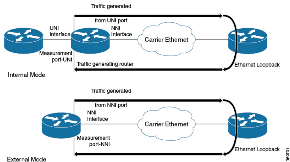
Figure 12: Traffic Generator Topology
