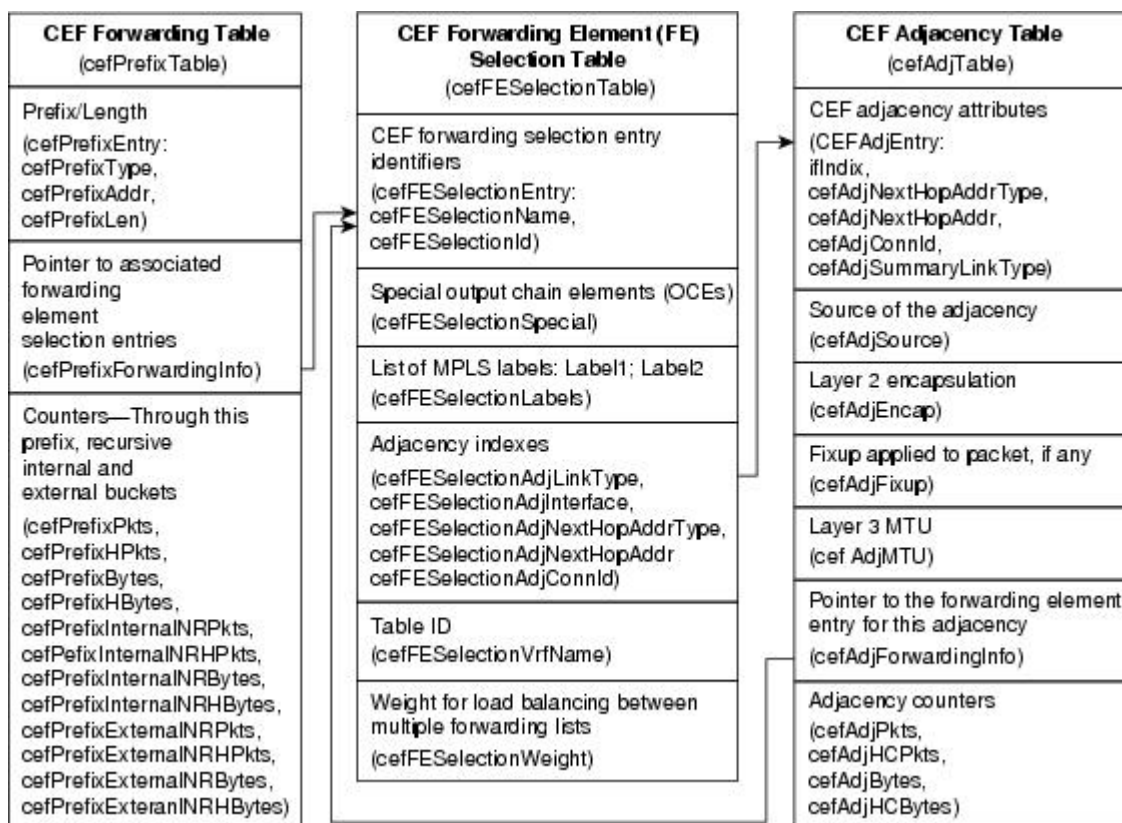
Figure 12: CISCO-CEF-MIB Main Tables, Table Contents, and Relationships
