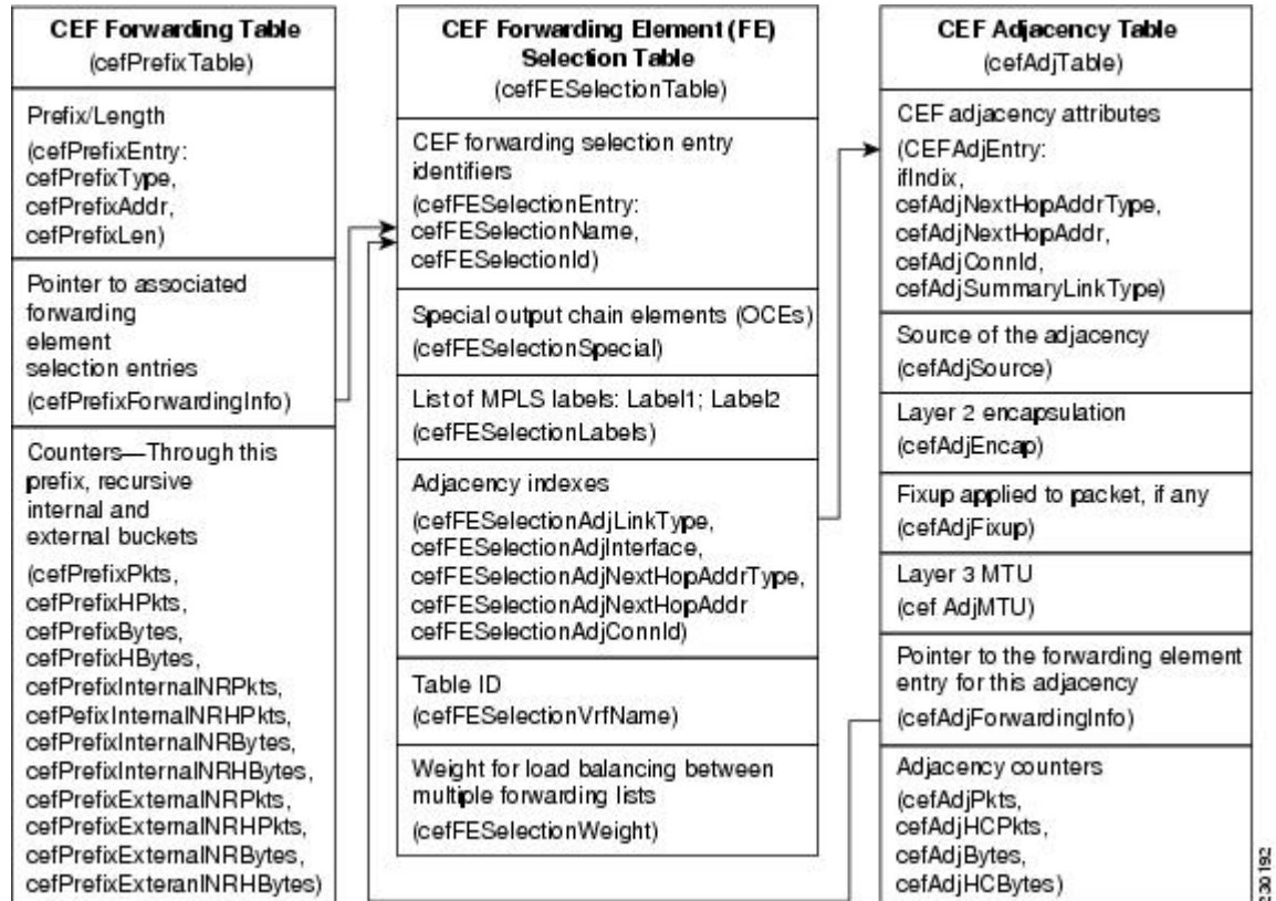
Figure 11: CISCO-CEF-MIB Main Tables, Table Contents, and Relationships
