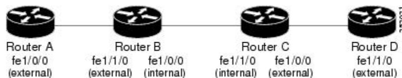
Figure 10: Sample Backbone Configuration
