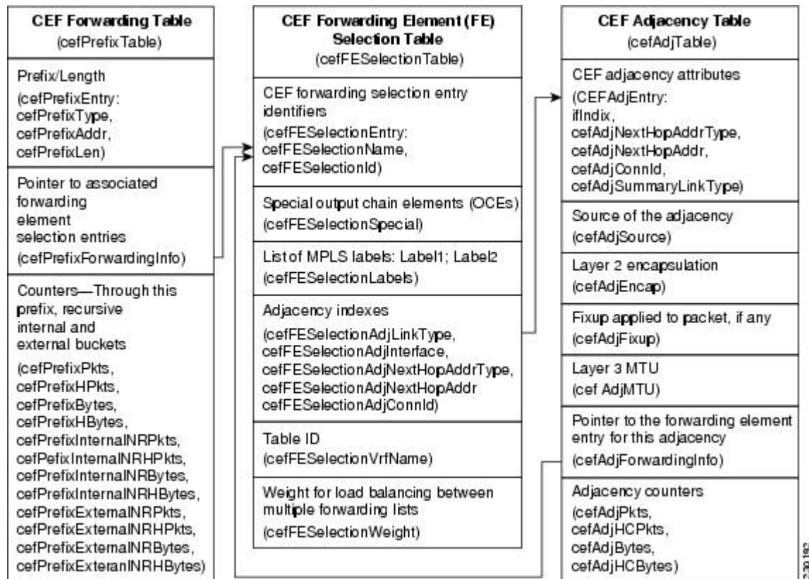
Figure 9 CISCO-CEF-MIB Main Tables, Table Contents, and Relationships
