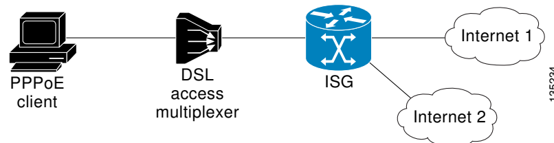
Figure 7 Flow-Based Policing
