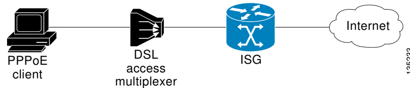
Figure 6 Session-Based Policing
