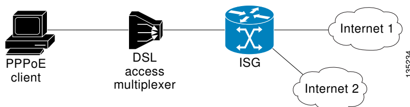
Figure 7 Flow-Based Policing
