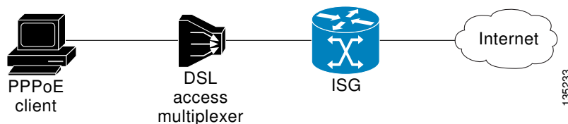
Figure 6 Session-Based Policing
