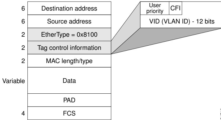
Figure 3 Tagging Scheme
