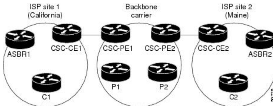
Figure 11: Sample BGP/MPLS Backbone Carrier Supporting an ISP
