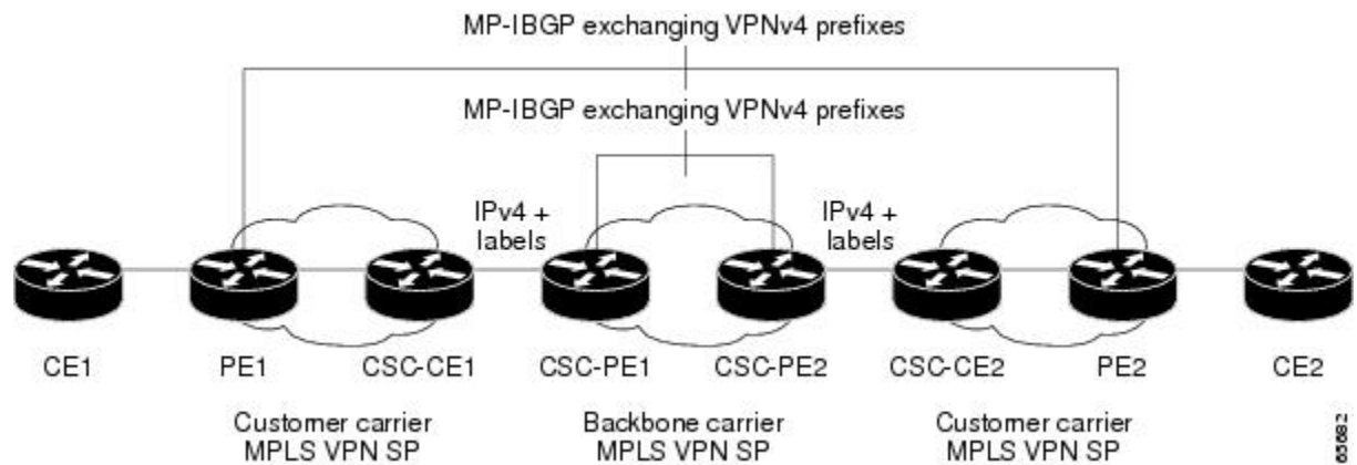
Figure 21: Network Where the Customer Carrier Is an MPLS VPN Service Provider
