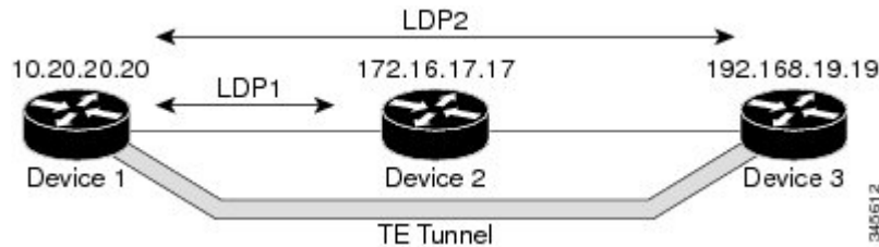
Figure 6: MPLS LDP Graceful Restart Configuration Example
