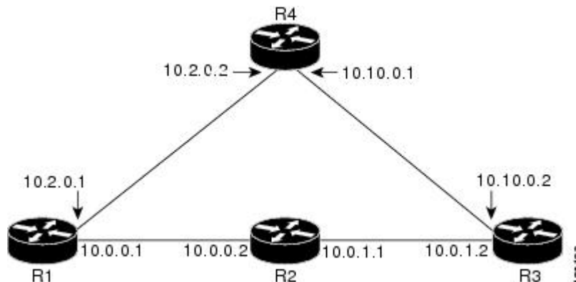
Figure 16 Network Topology--Path Protection
