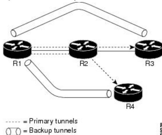
Figure 10 Backup Tunnels that Terminate at Different Destinations
