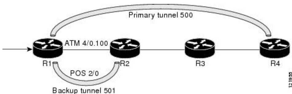
Figure 14 Protected LSPs
