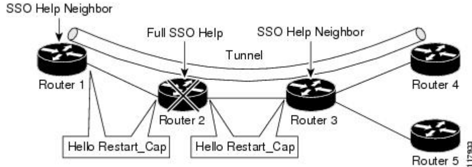
Figure 33 How Graceful Restart Works
