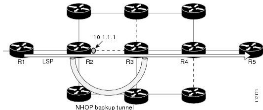
Figure 29 Autotunnel Backup for NHOP
