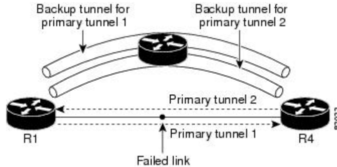
Figure 11 Backup Tunnels Share a Link
