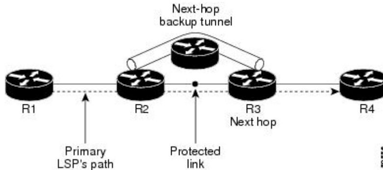
Figure 21 Next-Hop Backup Tunnel
