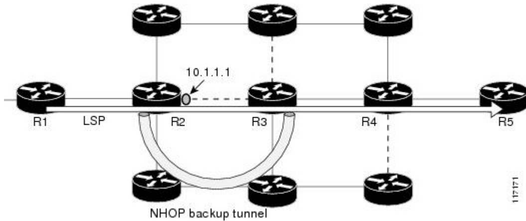
Figure 26 NHOP Backup Tunnel
