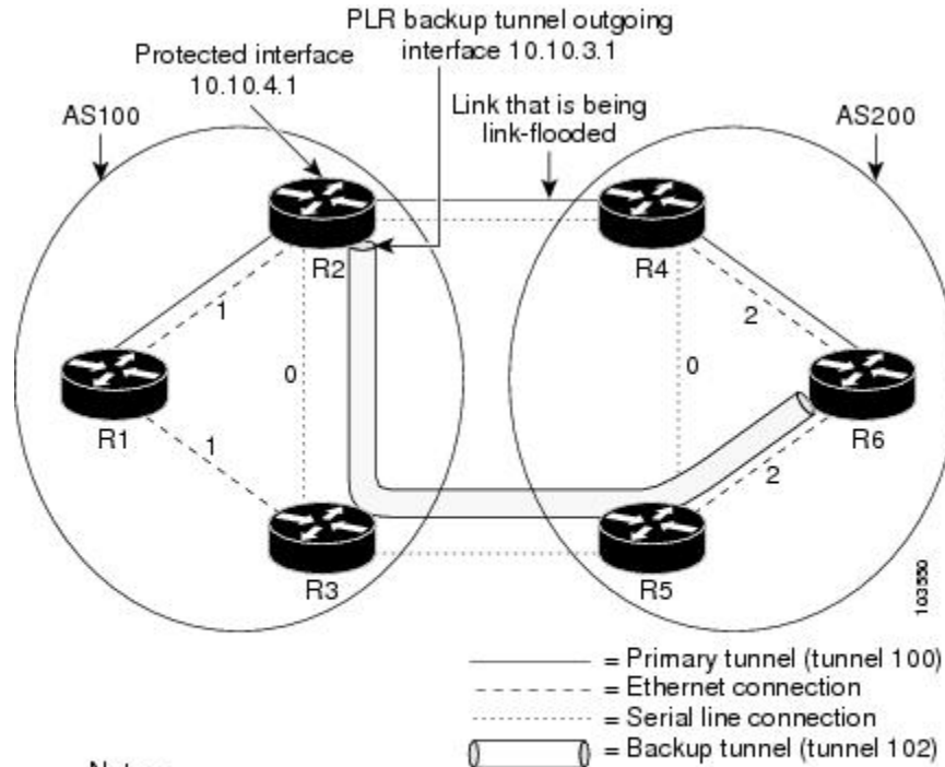
Figure 35: ASBR Node Protection
