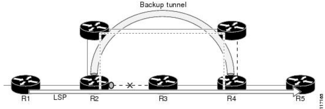
Figure 26: Backup Tunnel in the Same SRLG as the Interface It Is Protecting
