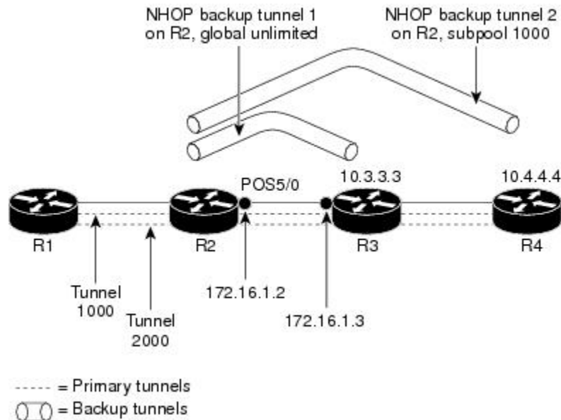
Figure 15: Backup Tunnels
