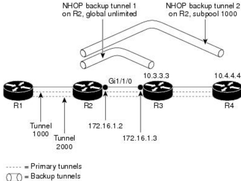
Figure 25: Backup Tunnels
